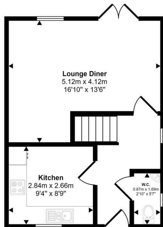
Ground Floor Approx 35 sq m / 378 sq ft
